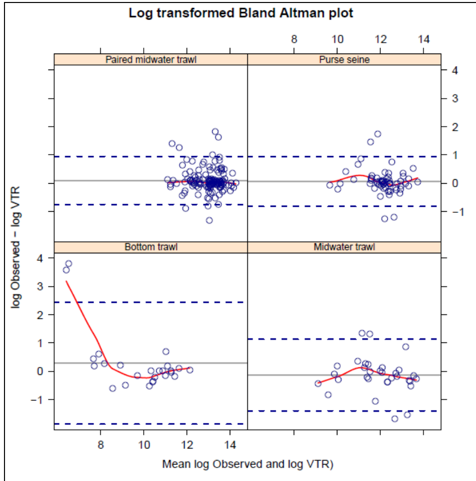
Figure B6: Log (observer/vtr) against mean log observer plus VTR. Excludes 2006 and observations where observer estimates=0. Gray line is the mean difference. Dashed blue lines are the mean +/- 2 standard deviations of the log (observer/VTR).
