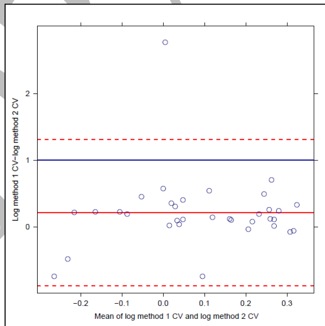
Figure C4: Comparison of river herring CV using Method 1 and Method 2 on log transformed scale. Solid red line is mean difference (Method 1-Method 2). Dashed lines are mean difference \pm 2 standard deviations.
